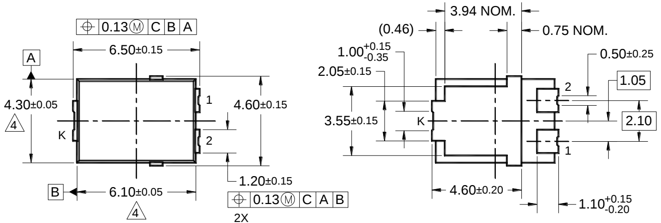
TO-277A (SMPC4.6U)
